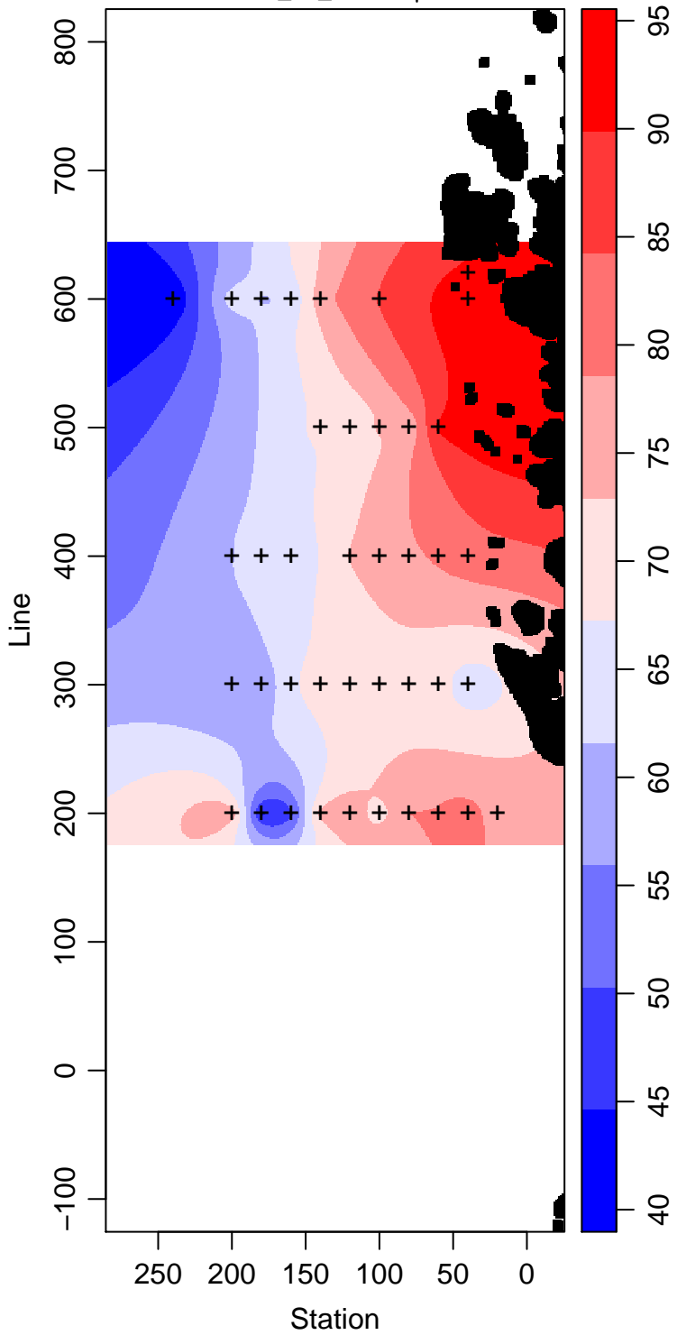
LMG05-01_40_Silicate \mu\text{ mol L}^{-1}
