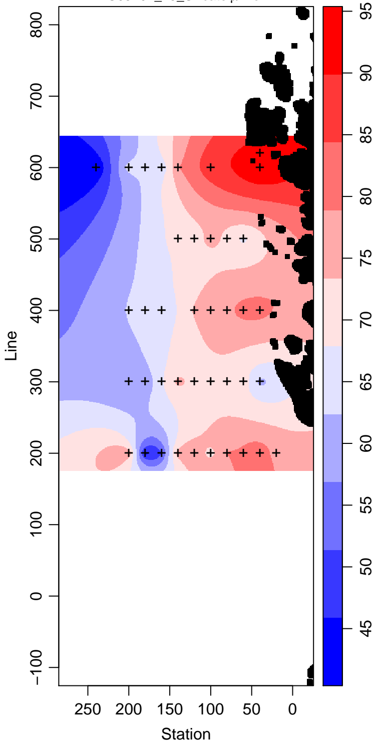
LMG05-01_45_Silicate \mu\text{ mol L}^{-1}
