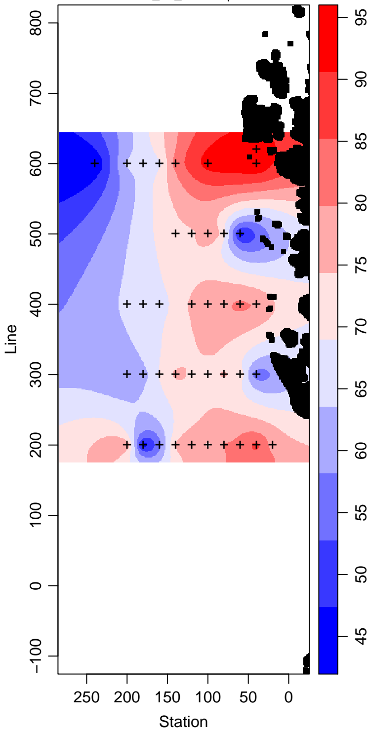
LMG05-01_55_Silicate \mu\text{ mol L}^{-1}
