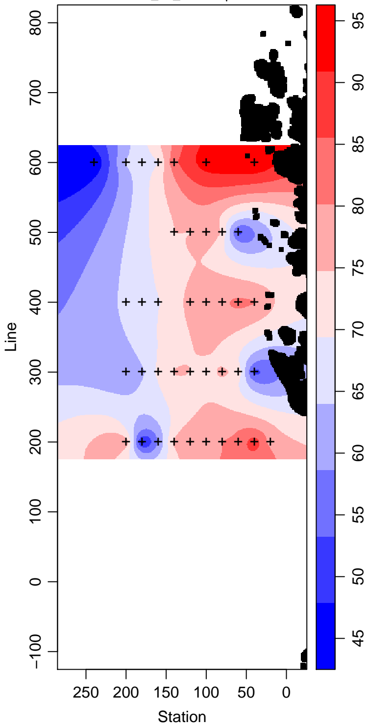
LMG05-01_60_Silicate \mu\text{ mol L}^{-1}
