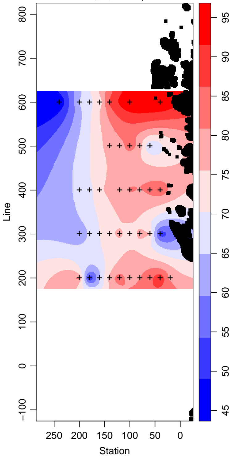
LMG05-01_70_Silicate \mu\text{ mol L}^{-1}
