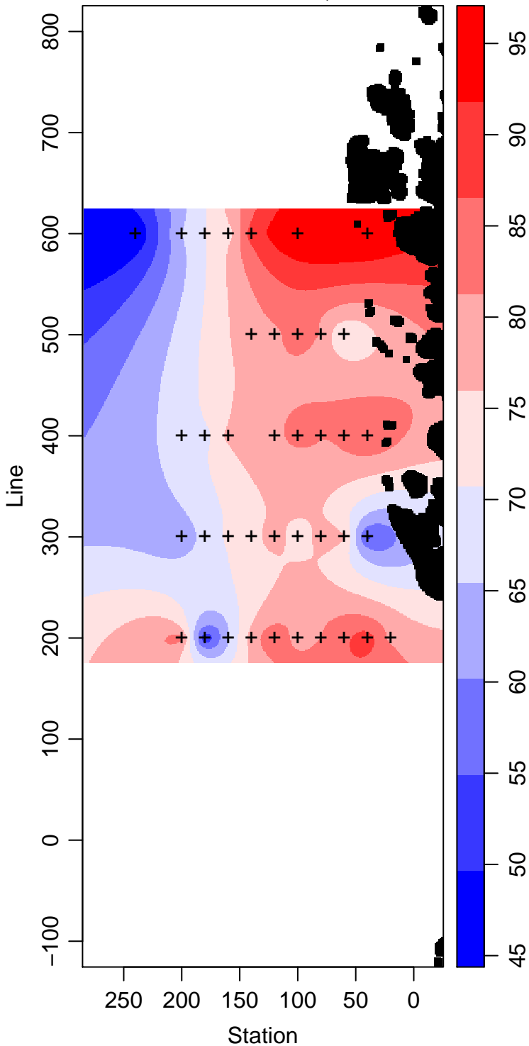
LMG05-01_75_Silicate \mu\text{ mol L}^{-1}
