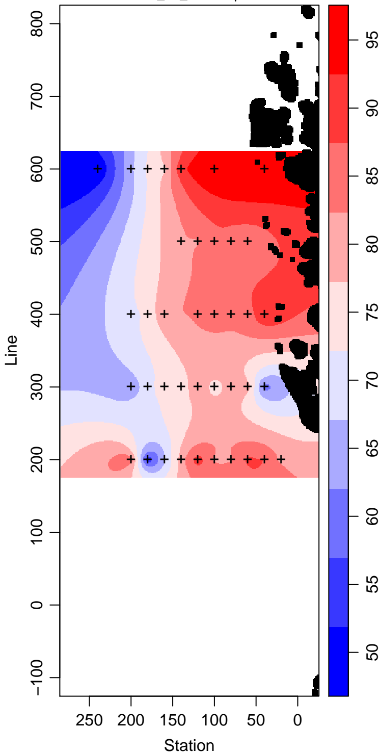
LMG05-01_85_Silicate \mu\text{ mol L}^{-1}
