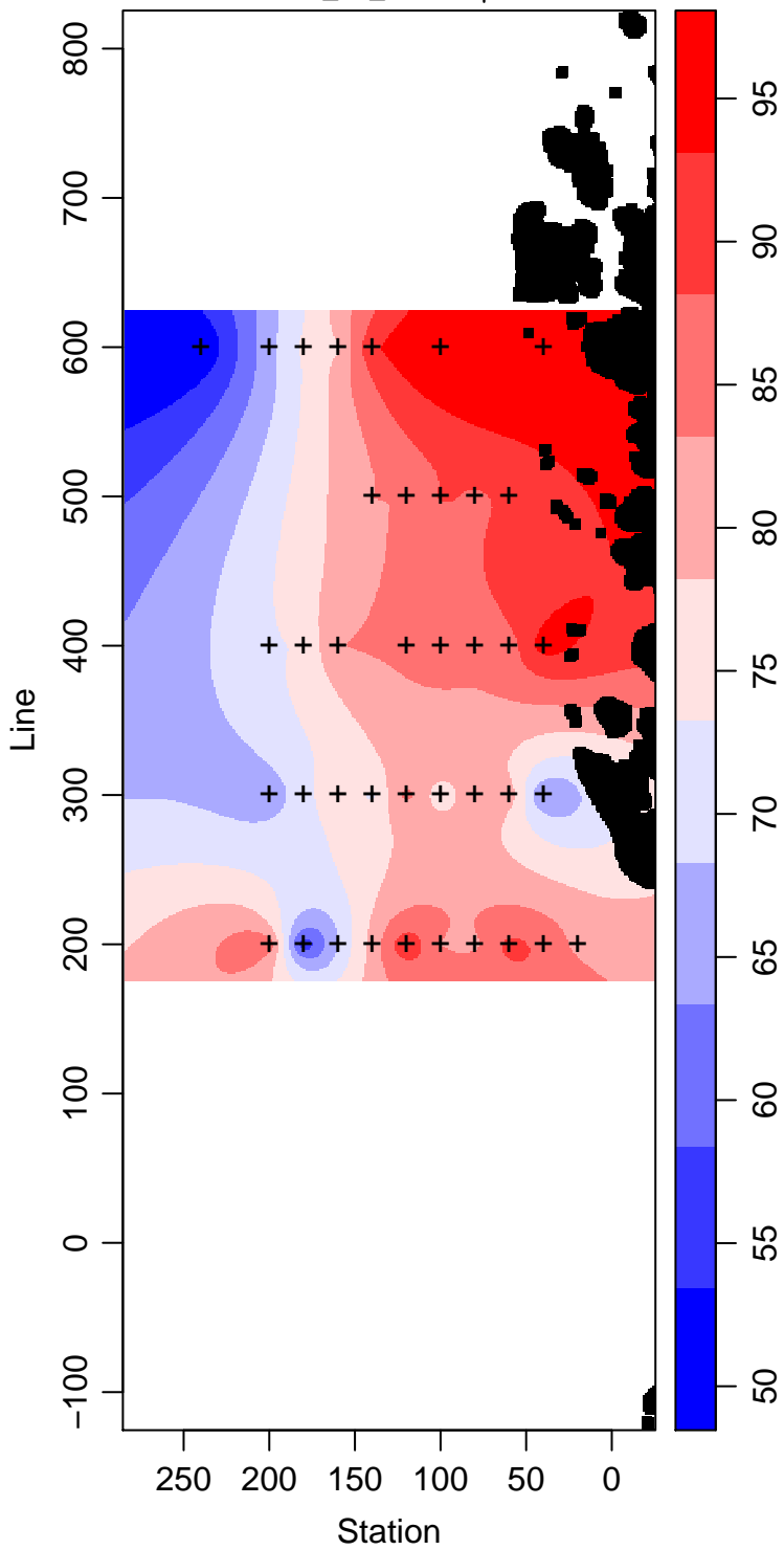
LMG05-01_90_Silicate \mu\text{ mol L}^{-1}
