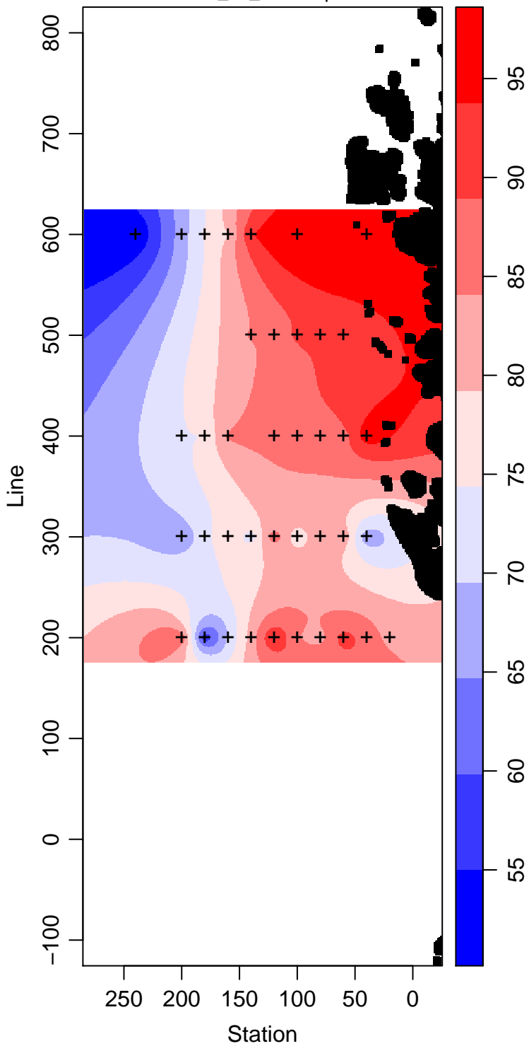
LMG05-01_95_Silicate \mu\text{ mol L}^{-1}
