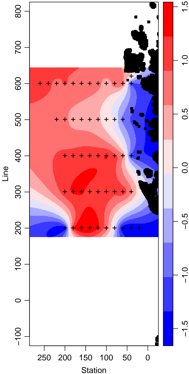
LMG05-01_15_Temperature ° Celsius
