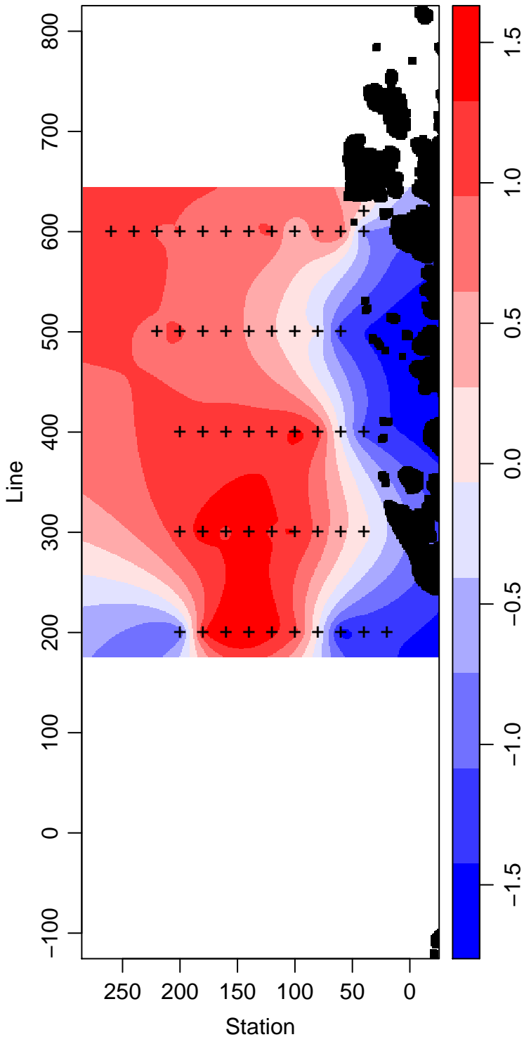
LMG05-01_1_Temperature ° Celsius
