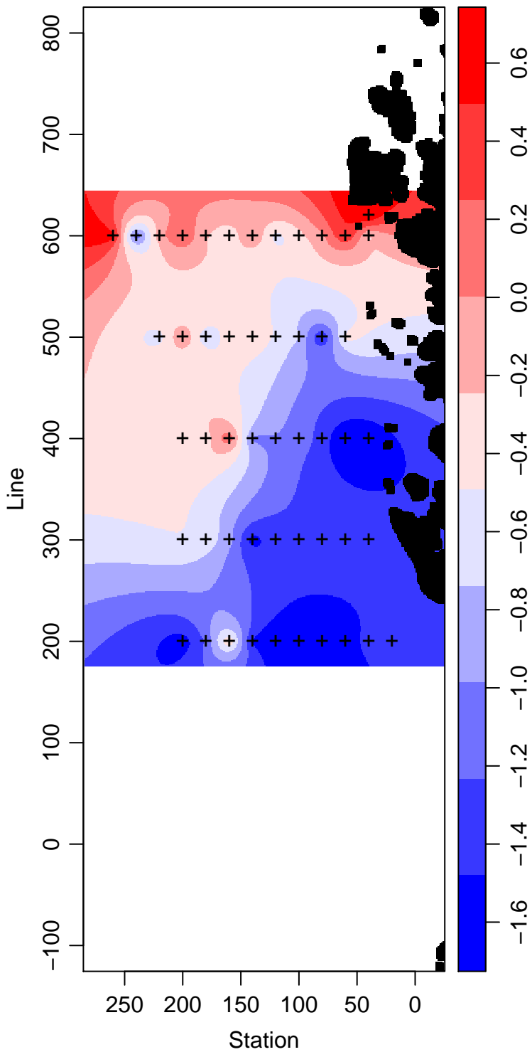
LMG05-01_55_Temperature ° Celsius
