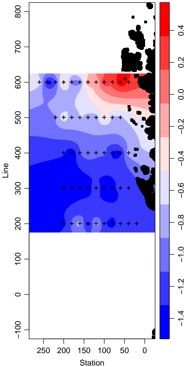
LMG05-01_85_Temperature ° Celsius
