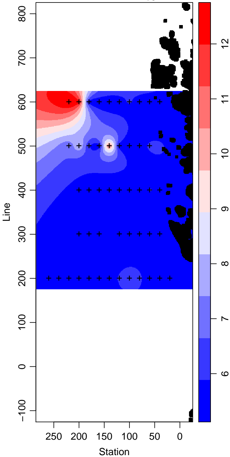
LMG06-01_10_Dissolved.Oxygen ml L -1
