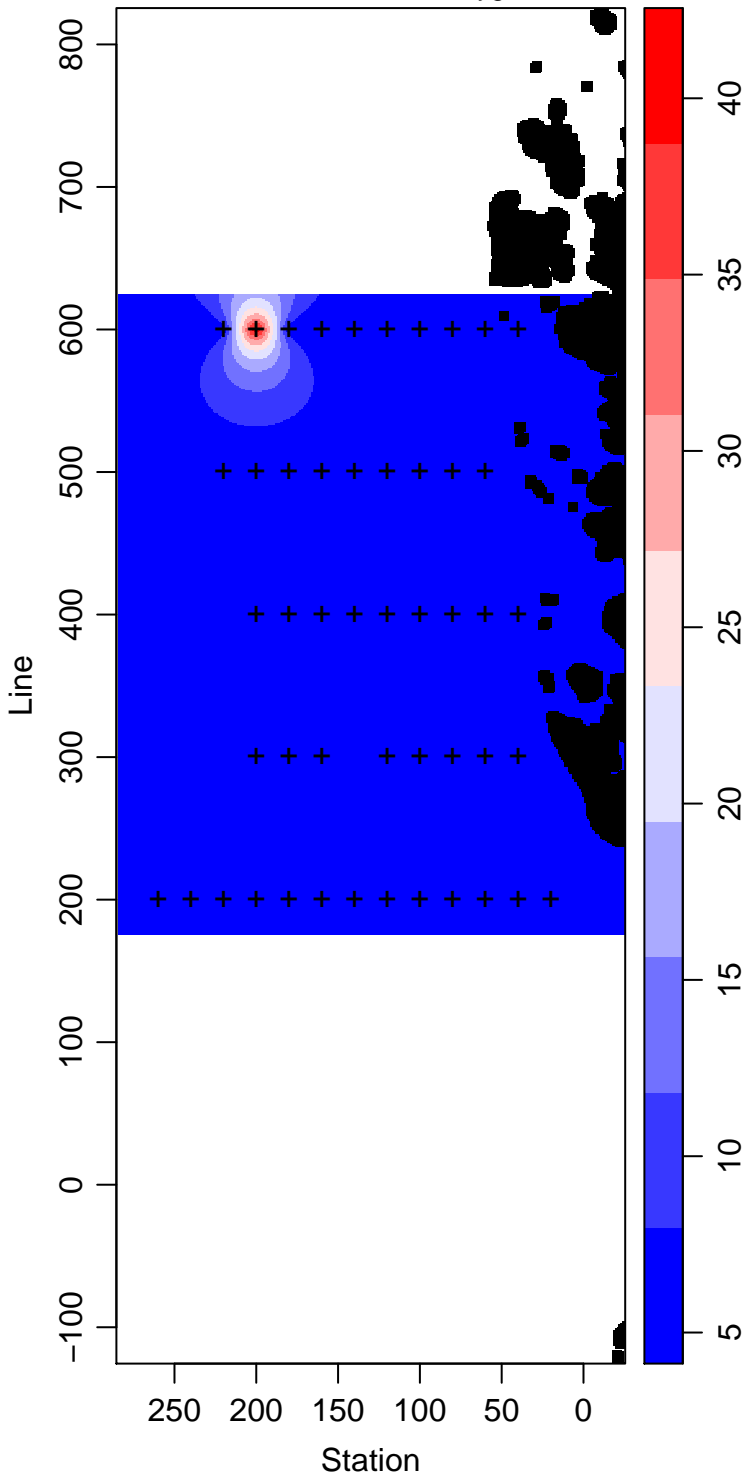
LMG06-01_45_Dissolved.Oxygen ml L -1
