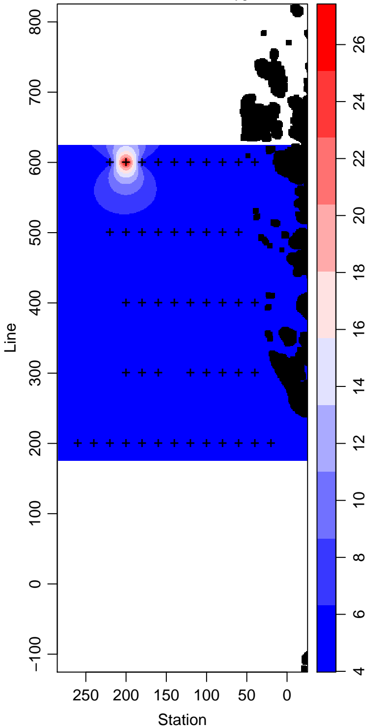
LMG06-01_55_Dissolved.Oxygen ml L -1
