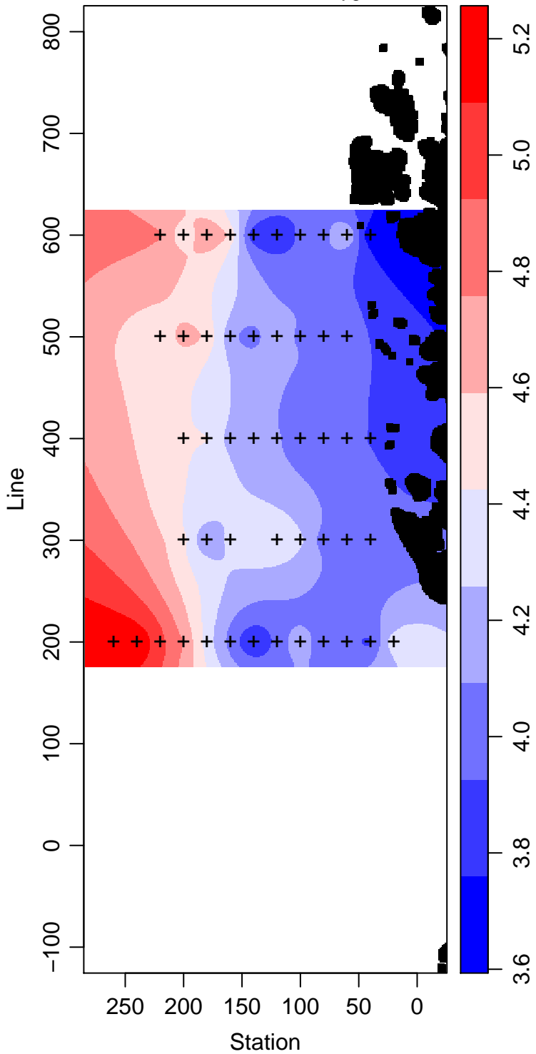
LMG06-01_80_Dissolved.Oxygen ml L -1
