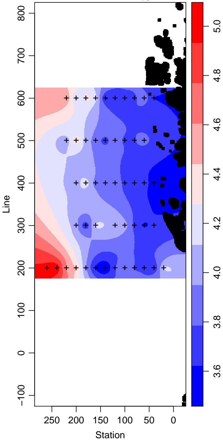
LMG06-01_95_Dissolved.Oxygen ml L -1
