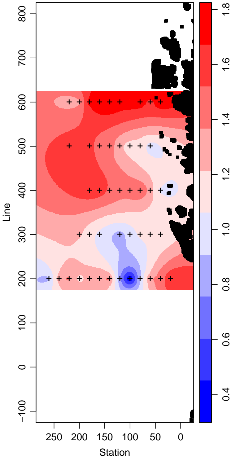
LMG06-01_10_Phosphate \mu\text{ mol L}^{-1}
