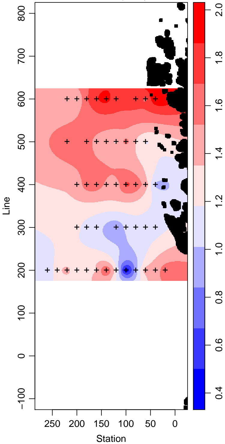
LMG06-01_15_Phosphate \mu\text{ mol L}^{-1}
