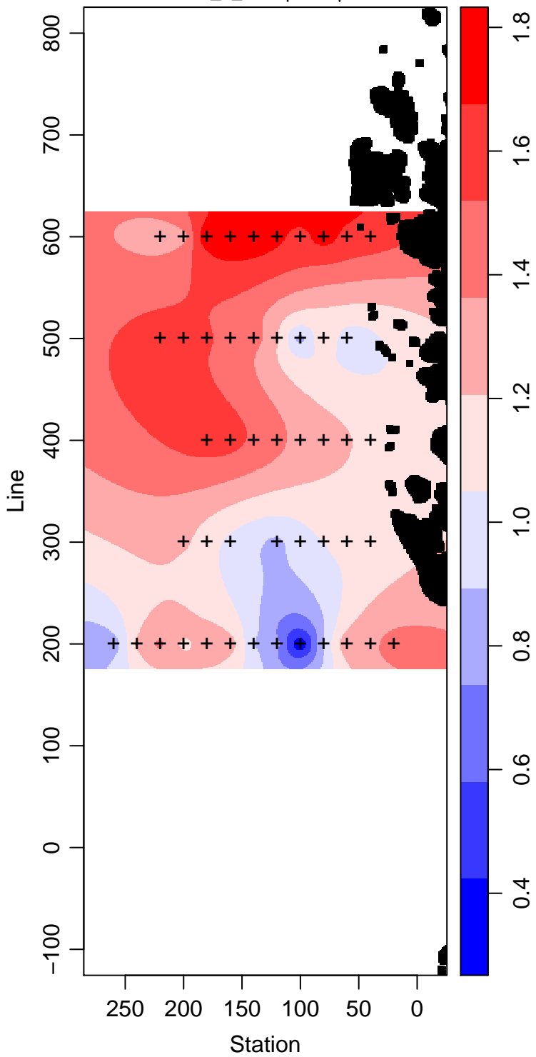
LMG06-01_1_Phosphate \mu\text{ mol L}^{-1}
