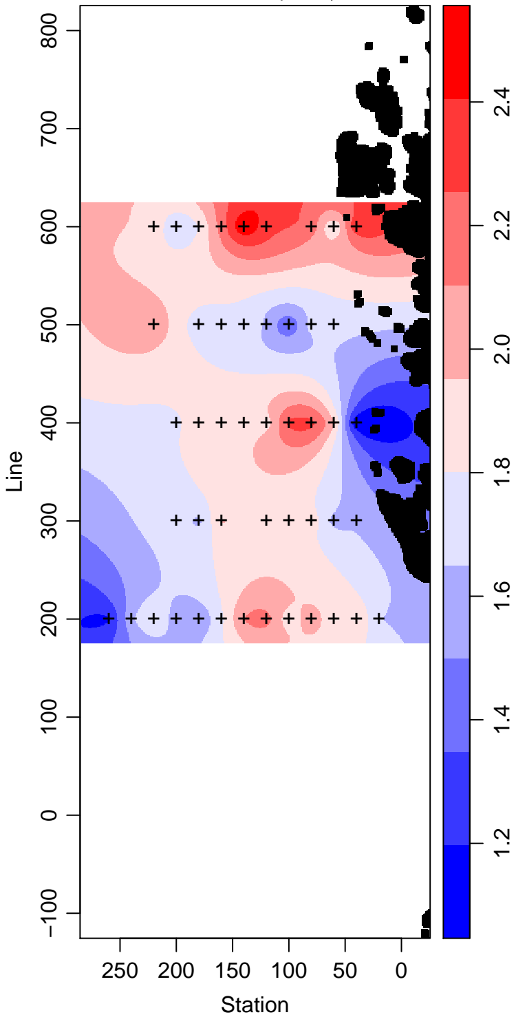
LMG06-01_35_Phosphate \mu\text{ mol L}^{-1}
