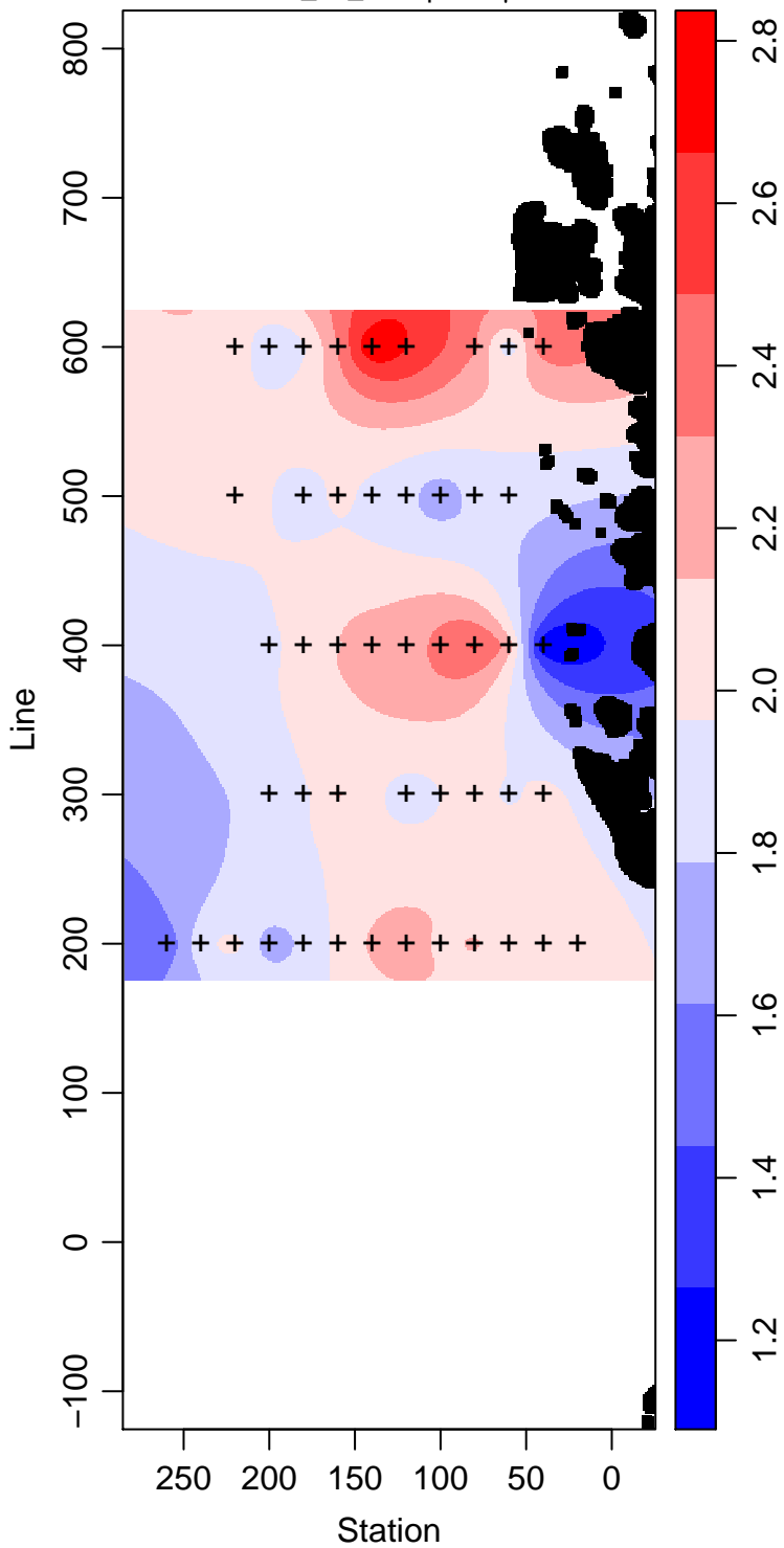
LMG06-01_45_Phosphate \mu\text{ mol L}^{-1}
