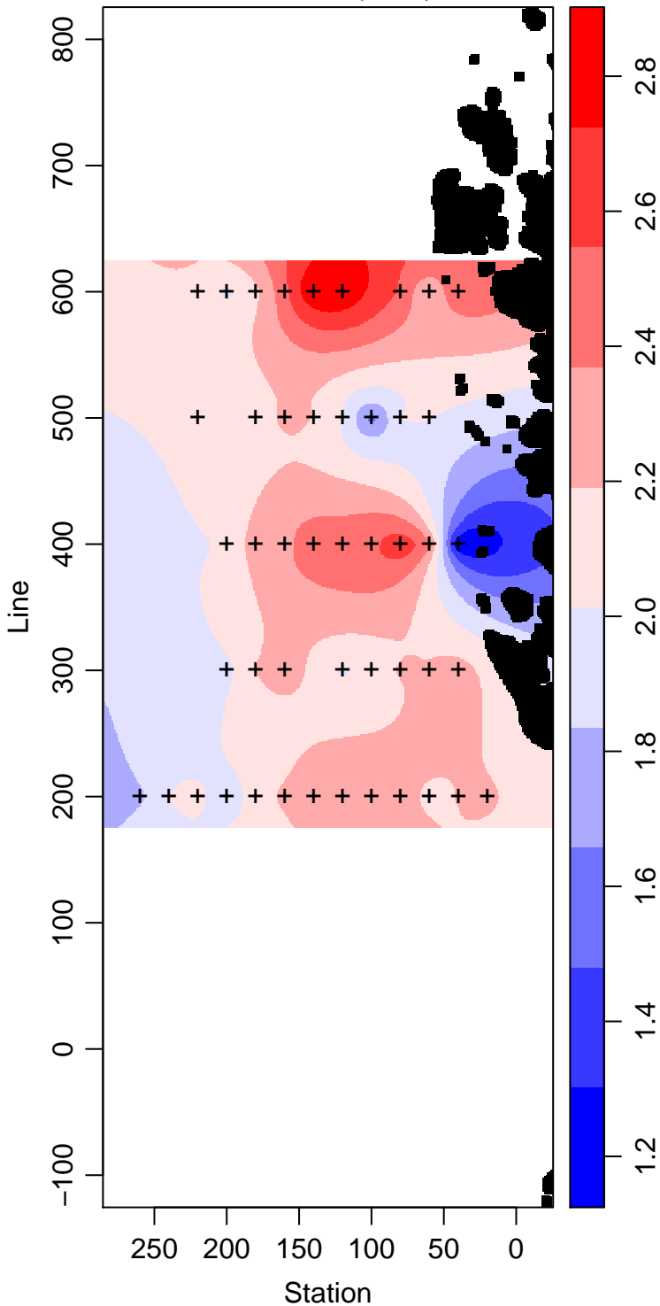
LMG06-01_60_Phosphate \mu\text{ mol L}^{-1}
