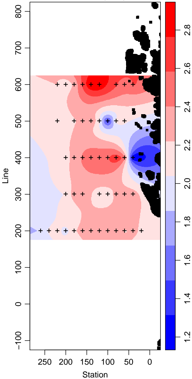
LMG06-01_70_Phosphate \mu\text{ mol L}^{-1}
