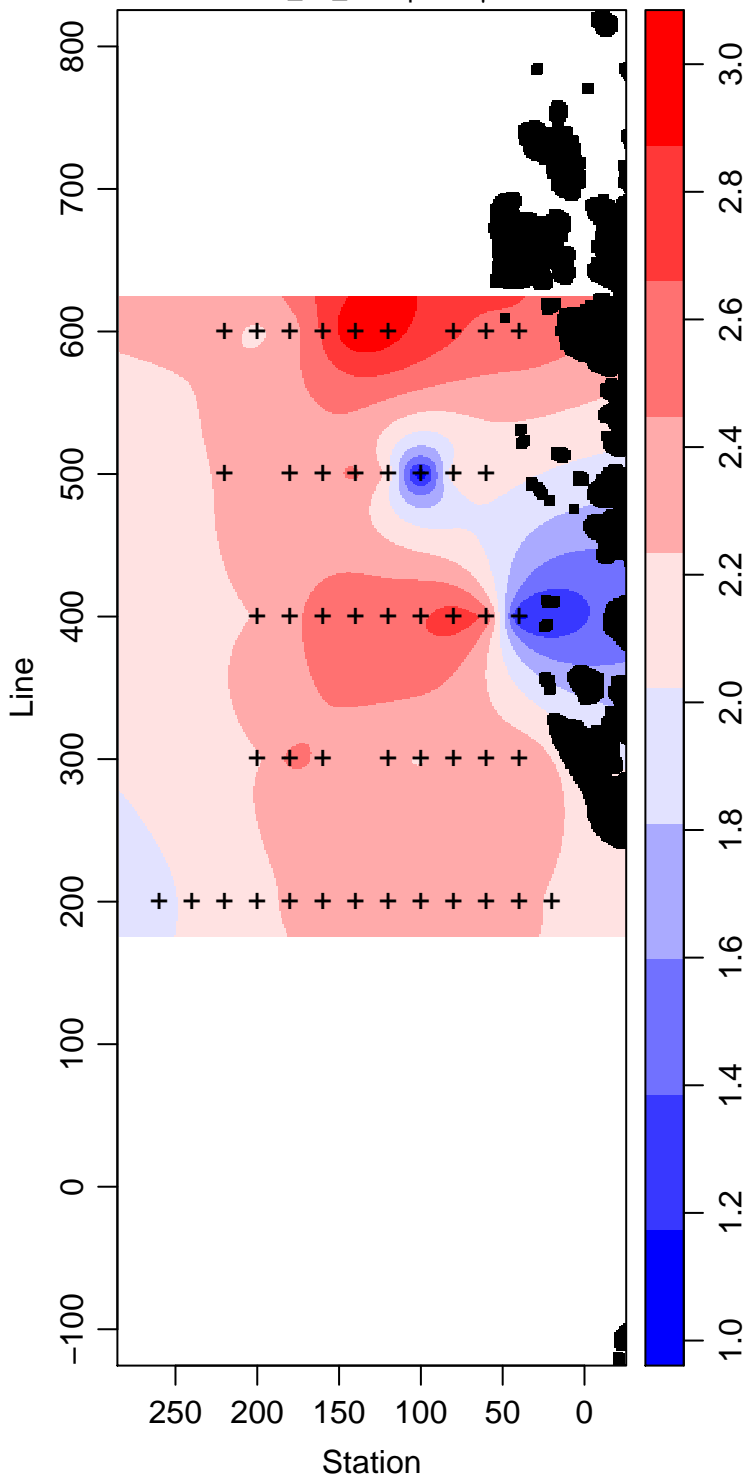
LMG06-01_85_Phosphate \mu\text{ mol L}^{-1}
