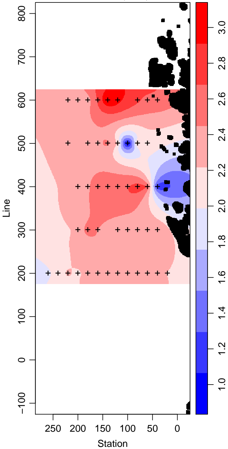
LMG06-01_90_Phosphate \mu\text{ mol L}^{-1}
