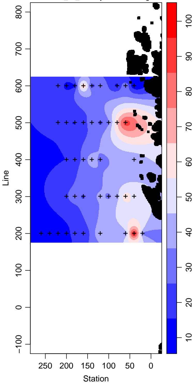
LMG06-01_20_Primary.Production mg m -3
