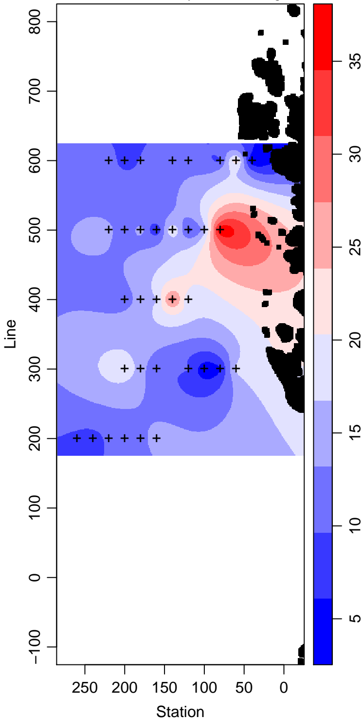
LMG06-01_30_Primary.Production mg m -3
