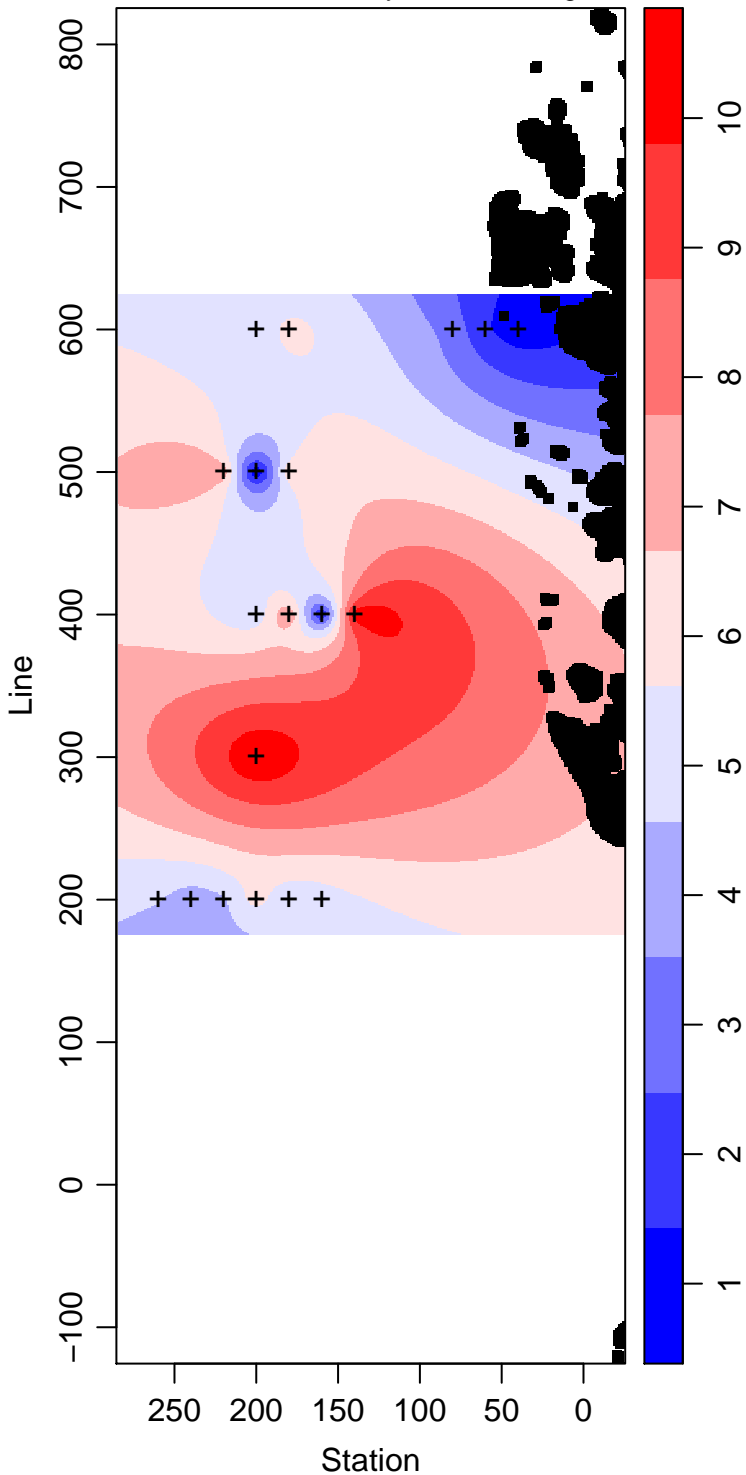
LMG06-01_45_Primary.Production mg m -3
