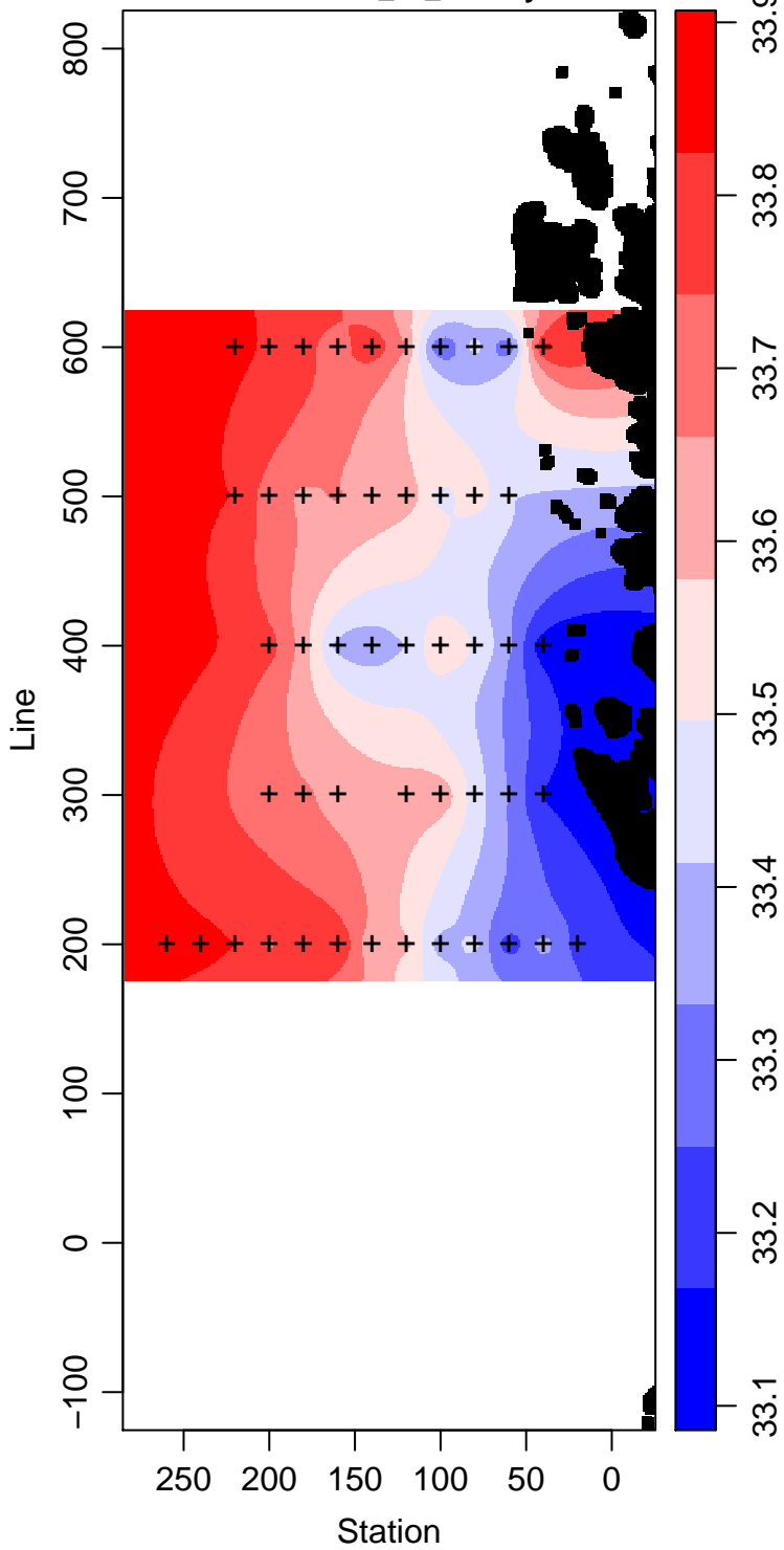
LMG06-01_25_Salinity
