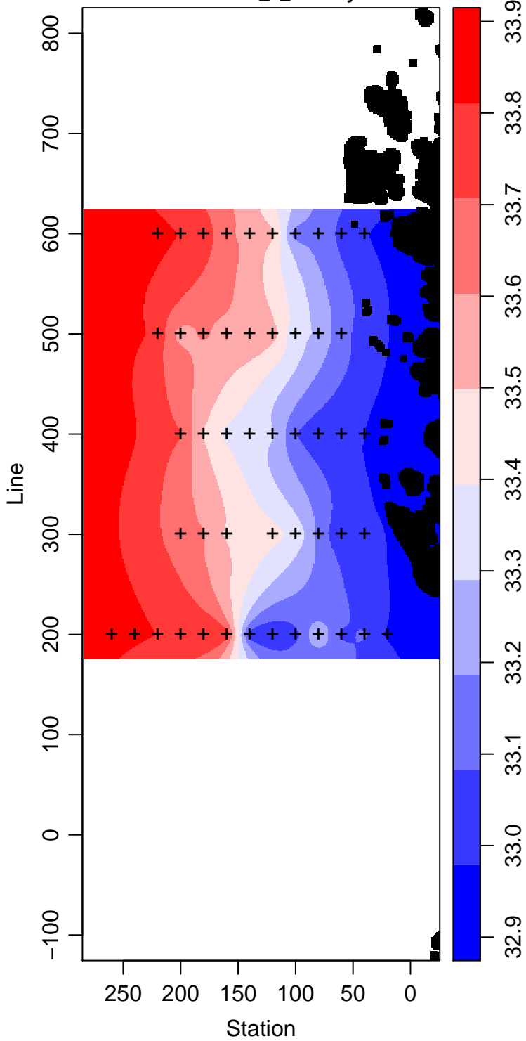
LMG06-01_5_Salinity
