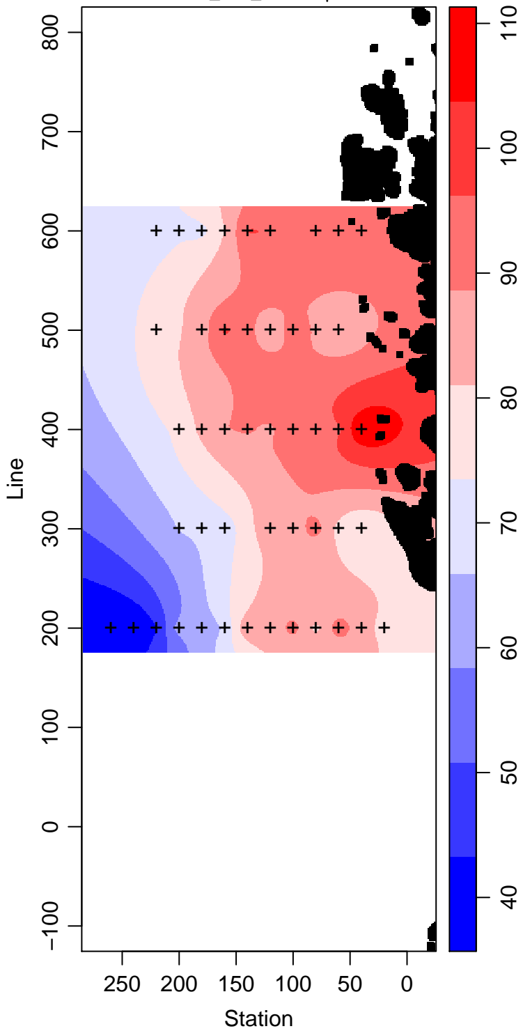
LMG06-01_100_Silicate \mu\text{ mol L}^{-1}
