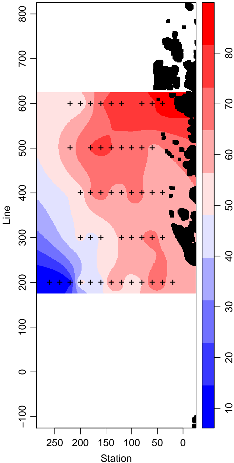
LMG06-01_15_Silicate \mu\text{ mol L}^{-1}
