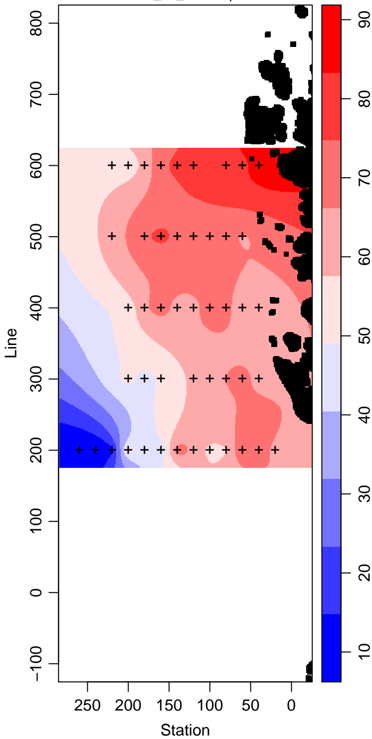
LMG06-01_20_Silicate \mu\text{ mol L}^{-1}
