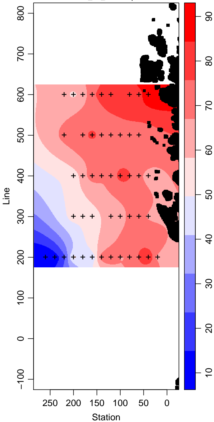
LMG06-01_30_Silicate \mu\text{ mol L}^{-1}
