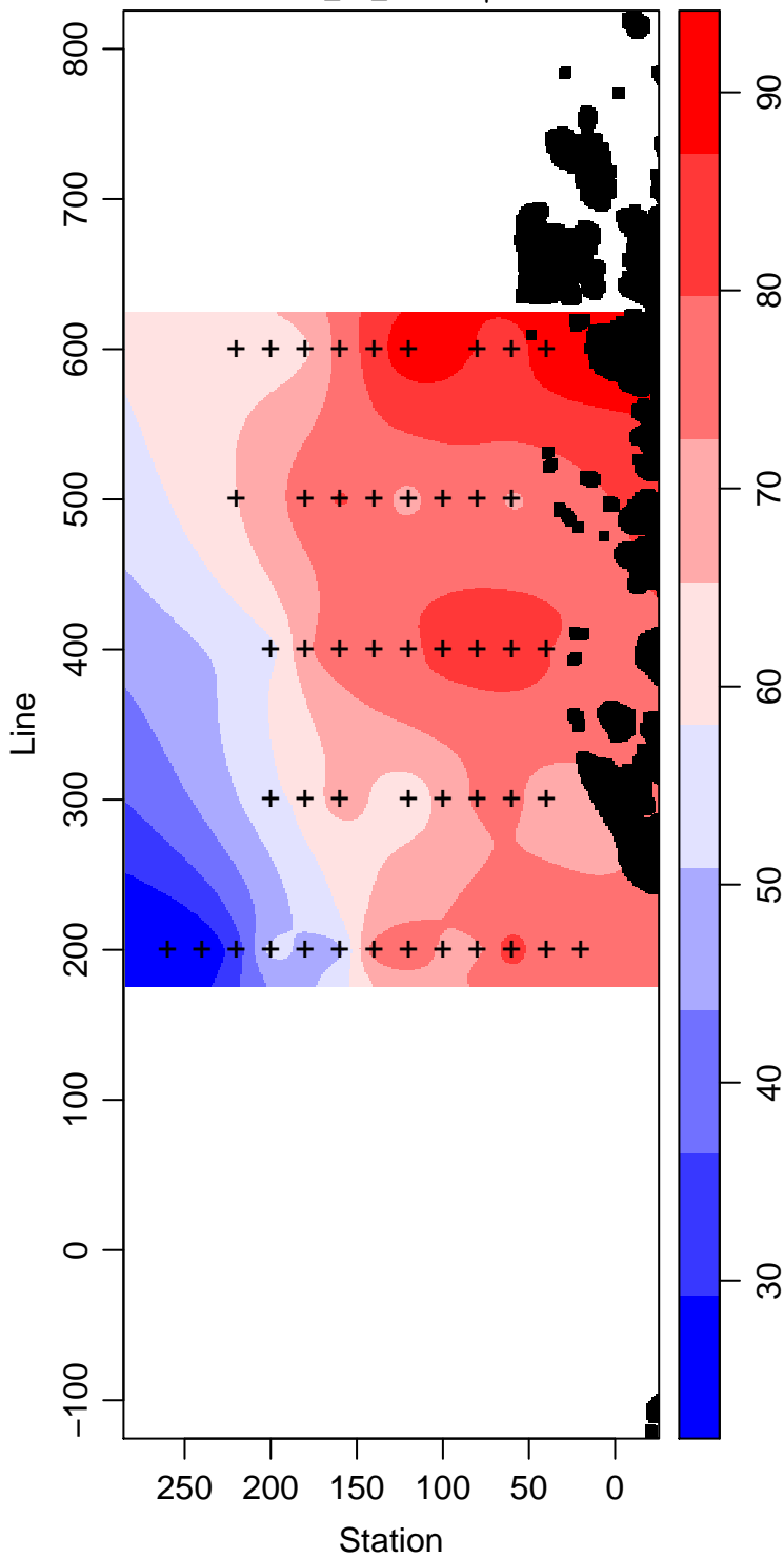
LMG06-01_50_Silicate \mu\text{ mol L}^{-1}
