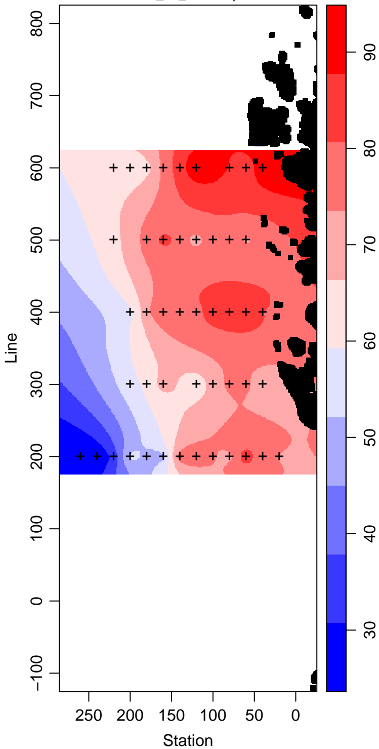
LMG06-01_55_Silicate \mu\text{ mol L}^{-1}
