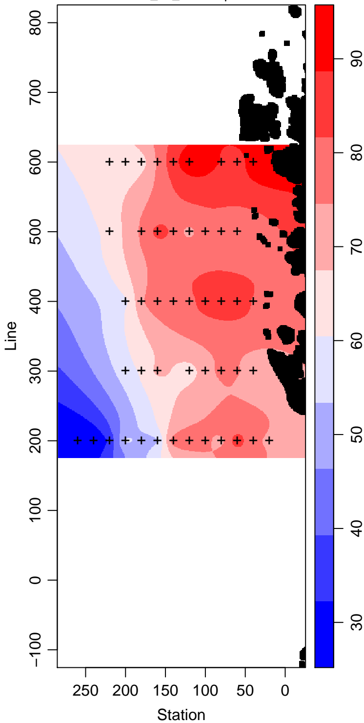
LMG06-01_60_Silicate \mu\text{ mol L}^{-1}
