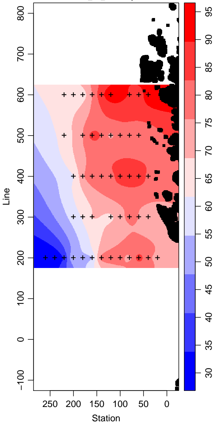
LMG06-01_65_Silicate \mu\text{ mol L}^{-1}
