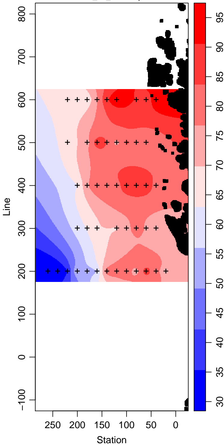
LMG06-01_70_Silicate \mu\text{ mol L}^{-1}
