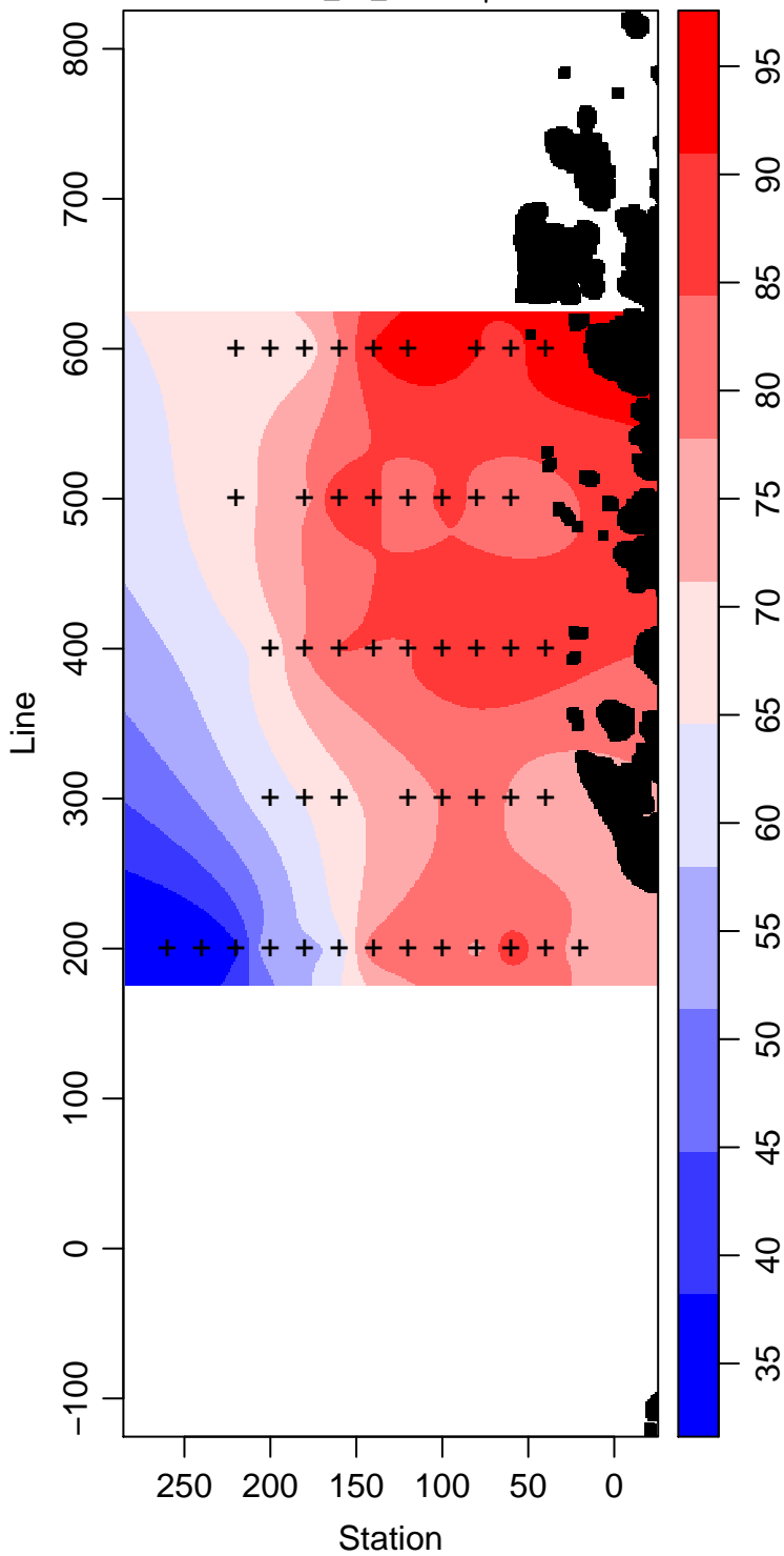
LMG06-01_80_Silicate \mu\text{ mol L}^{-1}
