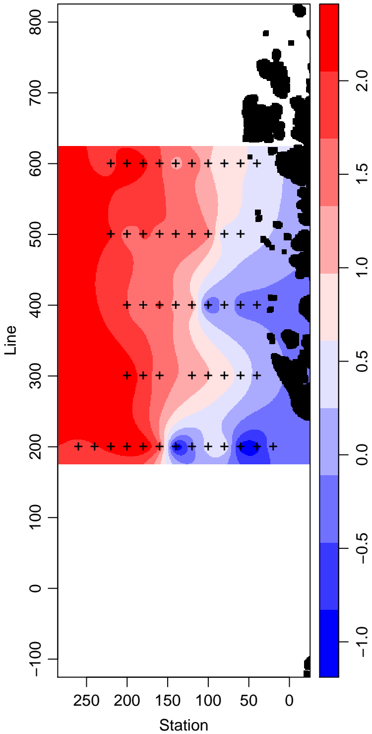
LMG06-01_15_Temperature ° Celsius
