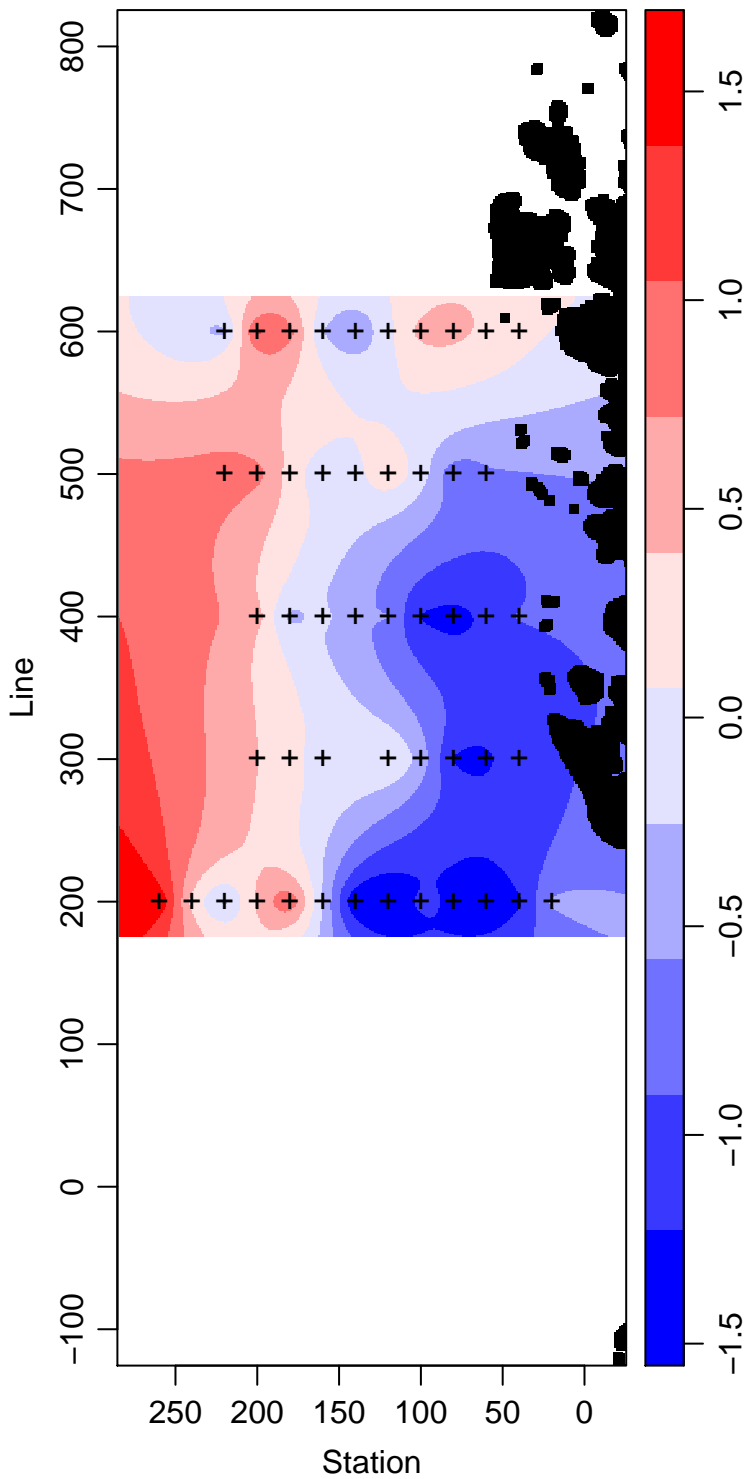
LMG06-01_40_Temperature ° Celsius
