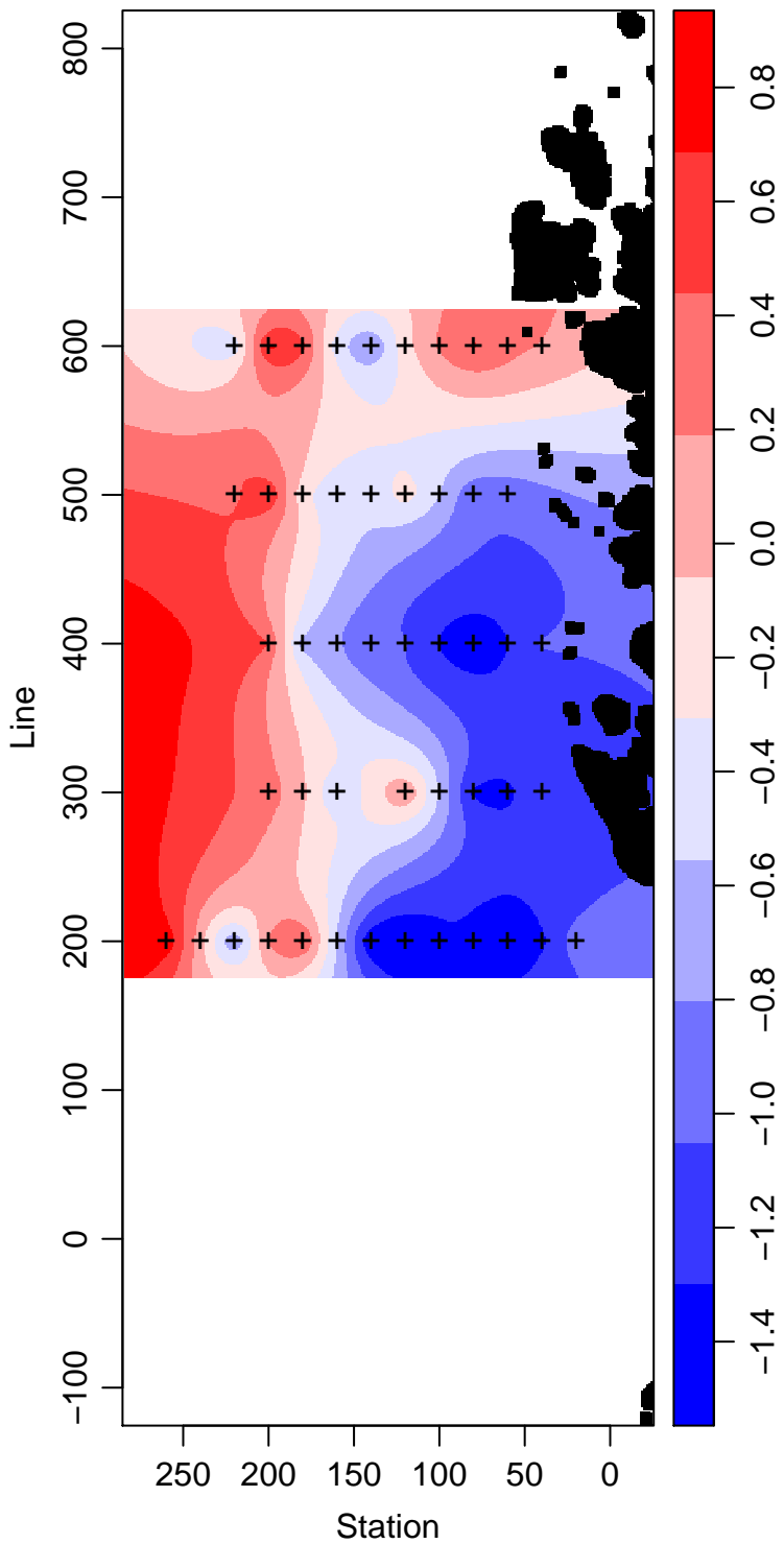
LMG06-01_45_Temperature ° Celsius
