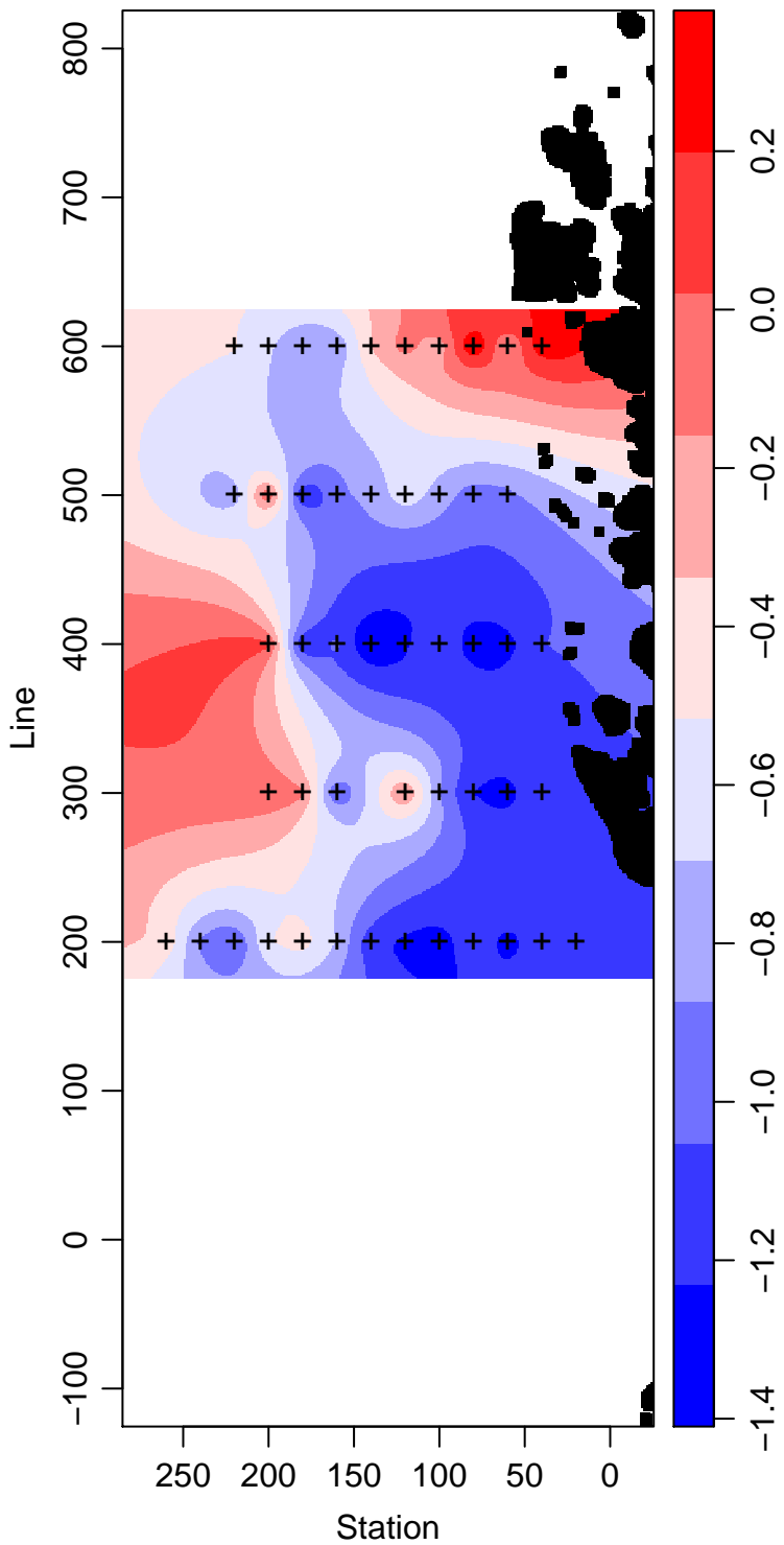
LMG06-01_65_Temperature ° Celsius
