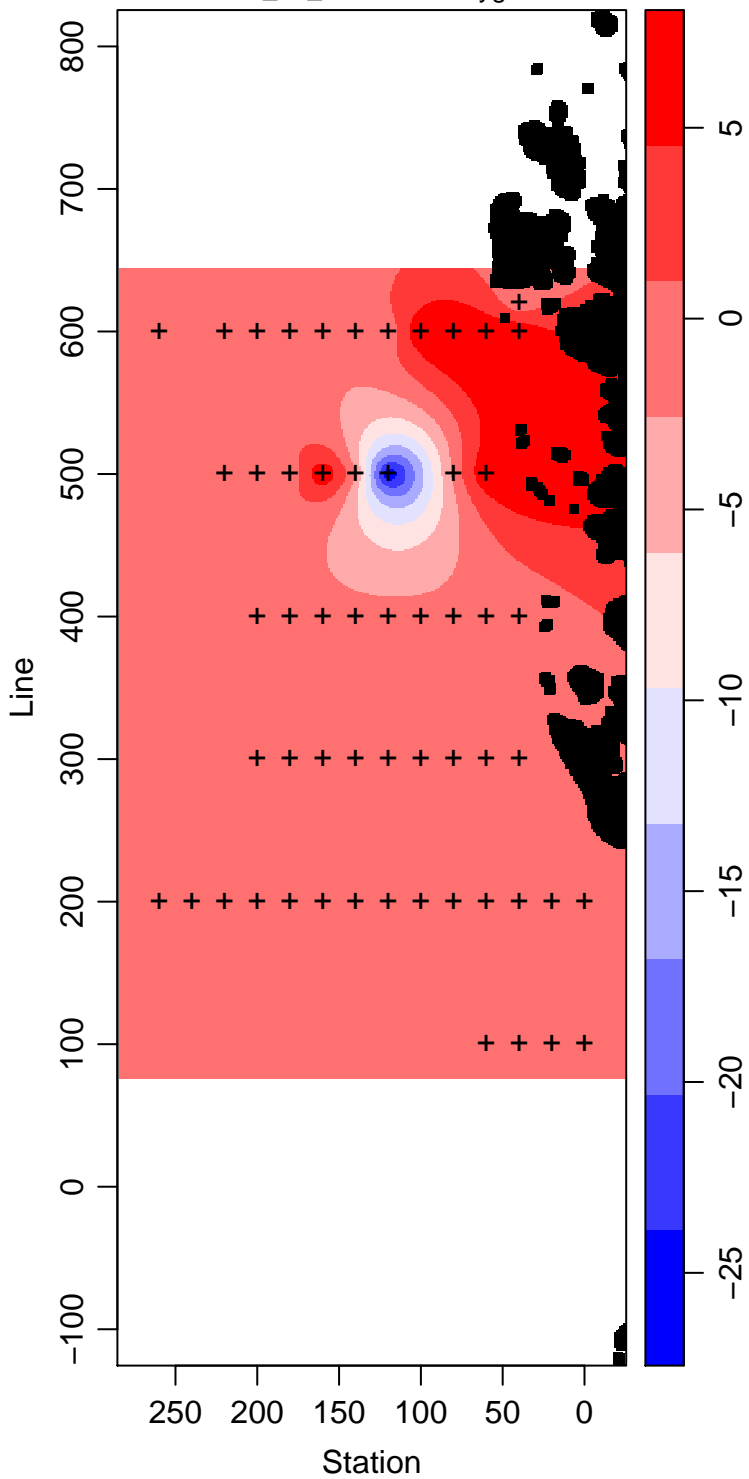
LMG07-01_30_Dissolved.Oxygen ml L -1
