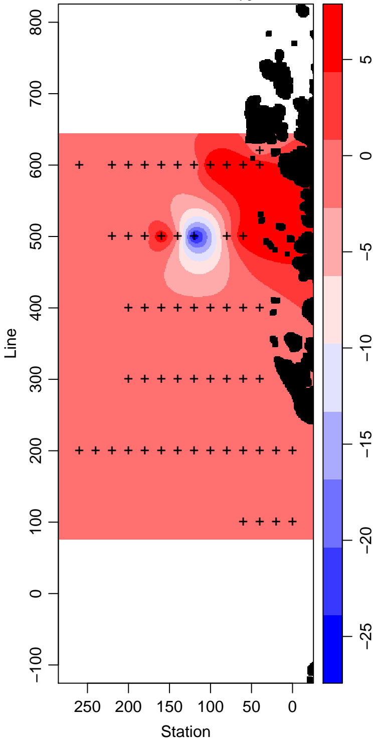
LMG07-01_40_Dissolved.Oxygen ml L -1
