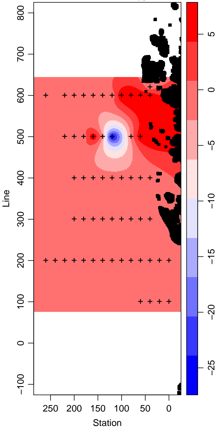
LMG07-01_50_Dissolved.Oxygen ml L -1
