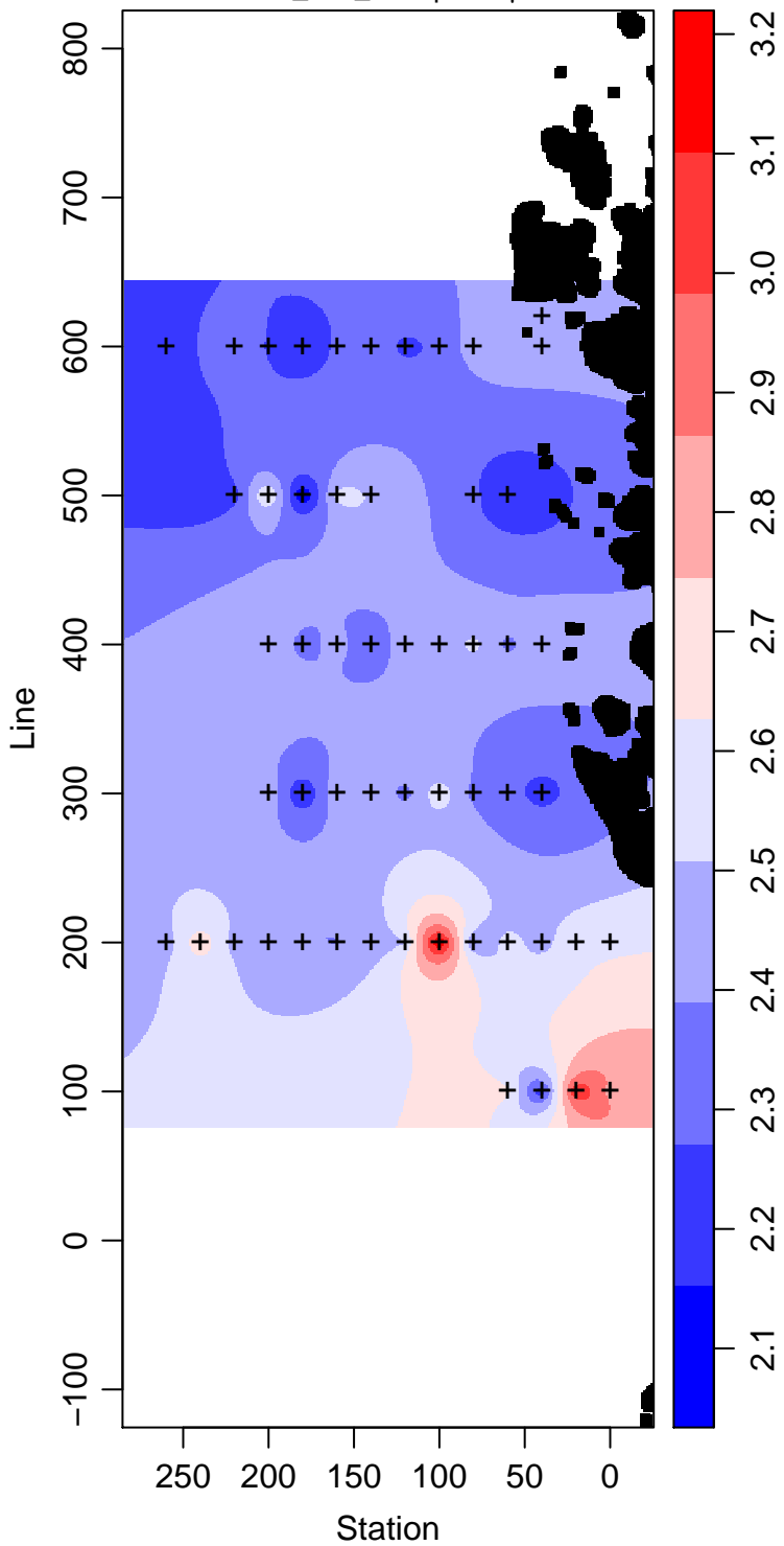
LMG07-01_100_Phosphate \mu\text{ mol L}^{-1}
